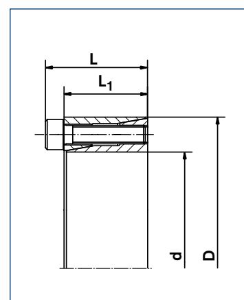
Locking Assembly RfN 7061 · Dimensions
