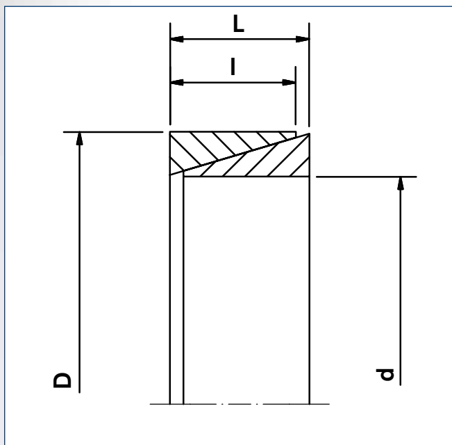
Locking Elements RINGFEDER® RfN 8006 stainless · Dimensions
