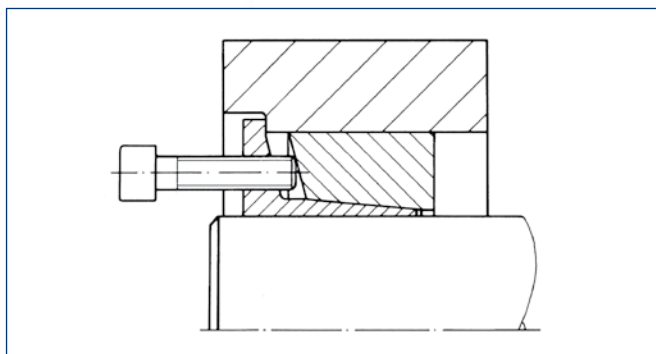
Removal of a Locking Assembly RfN 7013.1/7013.1-IN
