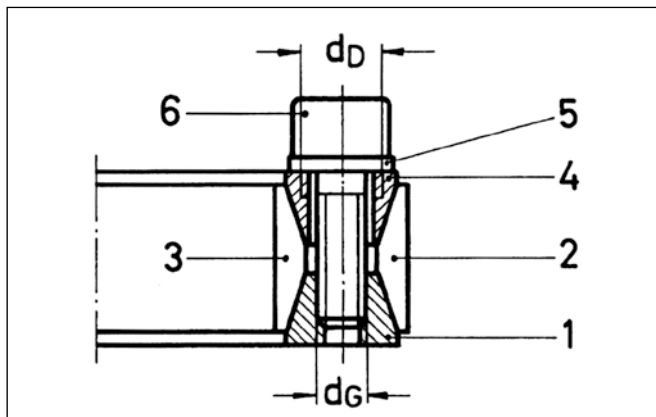
Locking Assembly RfN 7012-IN. Part description.
