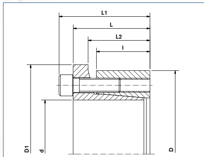
Locking Assembly RfN 7013.1-IN · Dimensions
