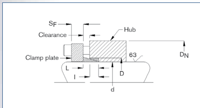
Hub bolted Clamp Plate (hub axially adjustable)
