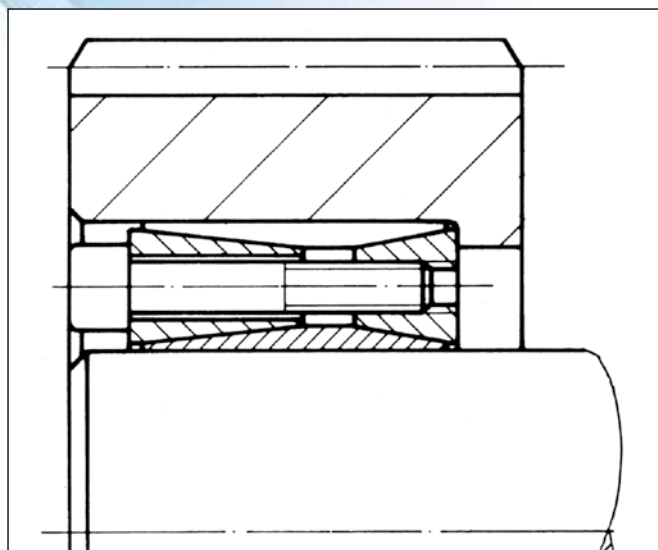
Locking Assembly not tightened
