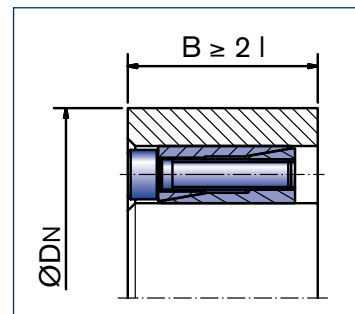
Locking Assembly RfN 7061 Typical installation
