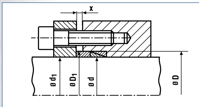
Locking Element RINGFEDER® RfN 8006 stainless · Typical installation
