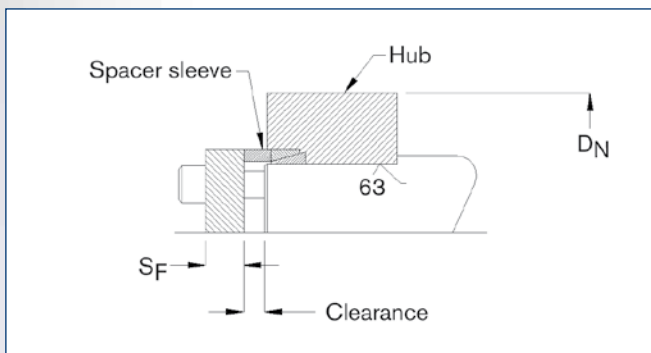
Shaft bolted Clamp Plate (hub axially fixed)
