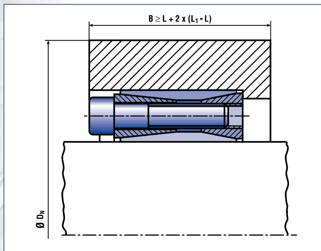
Locking Assembly RfN 7014 Typical installation
